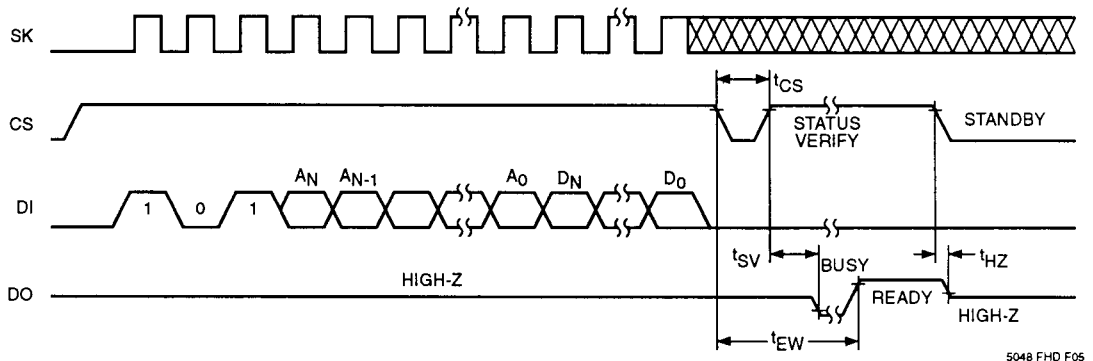
Figure 3. Write Instruction Timing (5)
